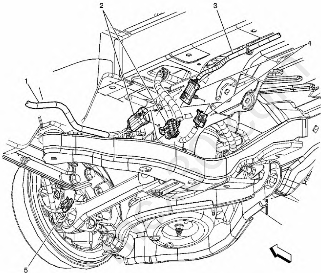
Fig. 7: View of Under the Rear of the Vehicle Harness Routing Courtesy of GENERAL MOTORS CORP.
