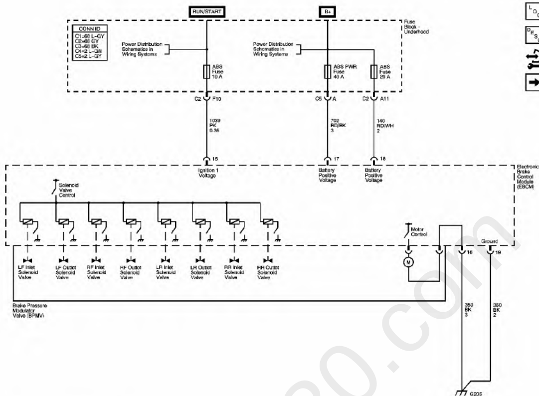
Fig. 1: Power, Ground Courtesy of GENERAL MOTORS CORP.
