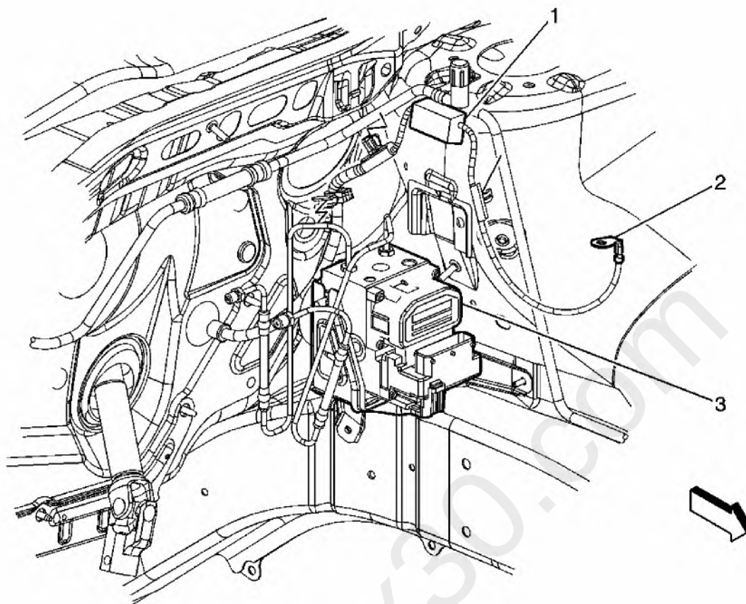
Fig. 5: View of Electronic Power Steering Harness, Underhood Side Harness Routing Courtesy of GENERAL MOTORS CORP.
