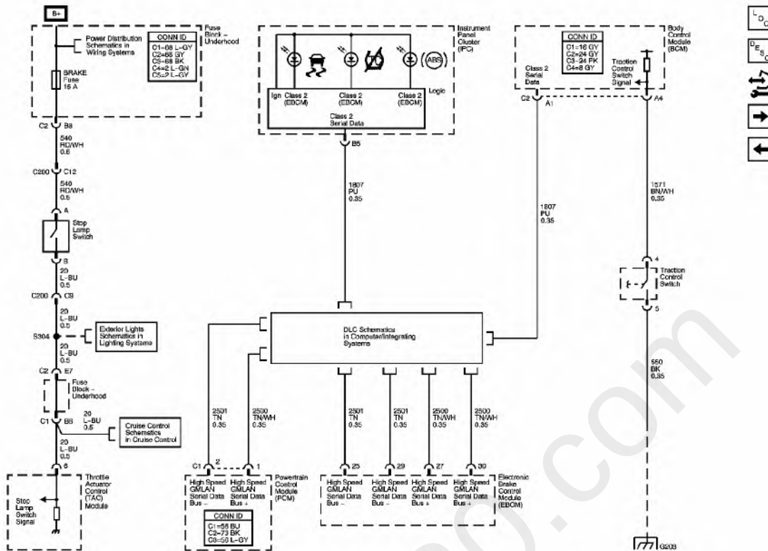
Fig. 2: Indicators, TC Switch Courtesy of GENERAL MOTORS CORP.
