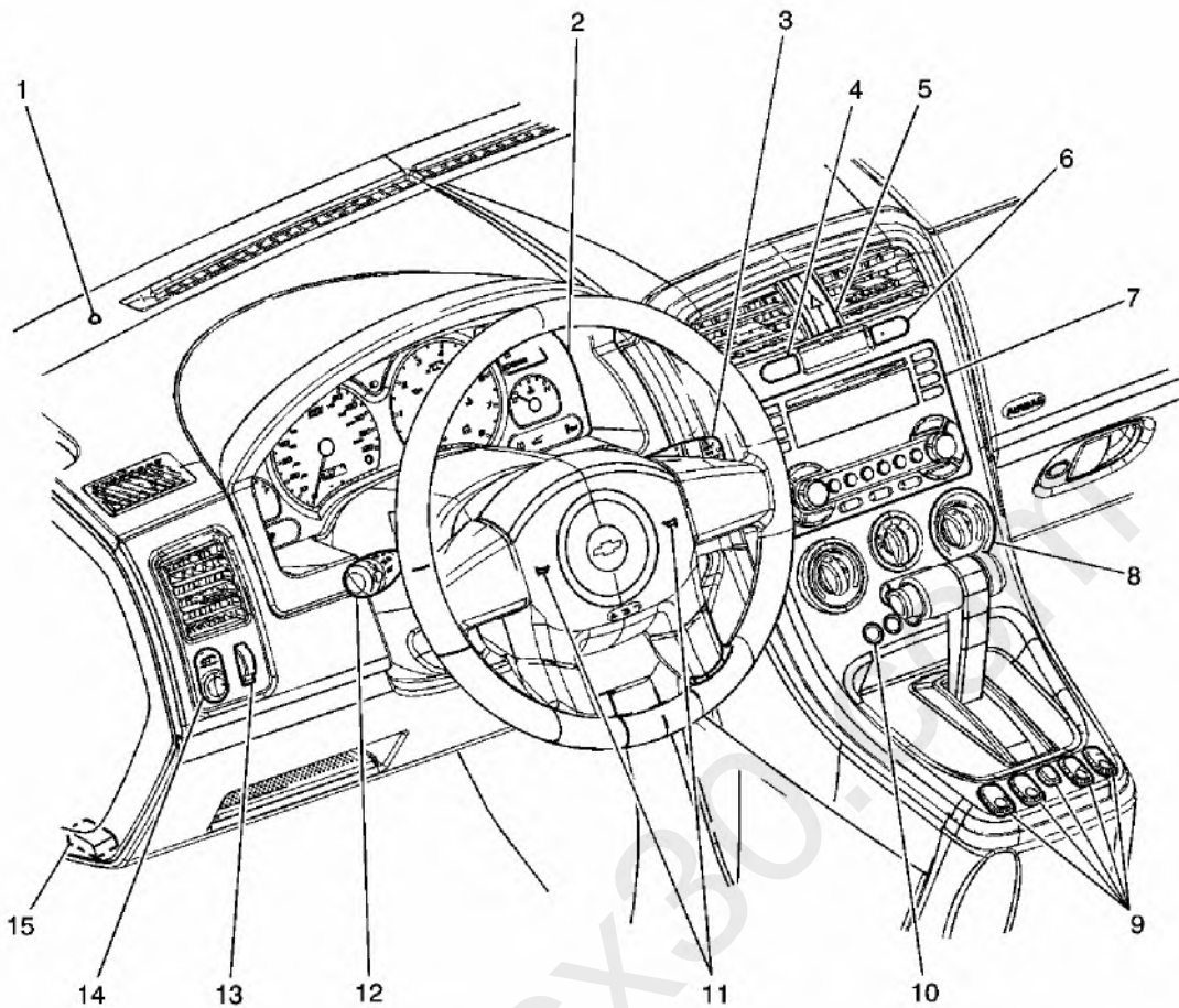
Fig. 6: Left Side of the I/P Courtesy of GENERAL MOTORS CORP.
