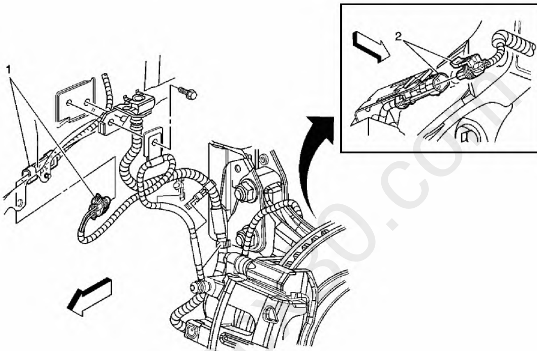
Fig. 4: View of LF Suspension Harness Routing Courtesy of GENERAL MOTORS CORP.
